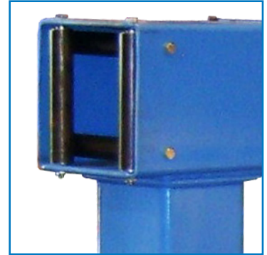
6" Capacity Guide with Bearing Mounted Rollers
